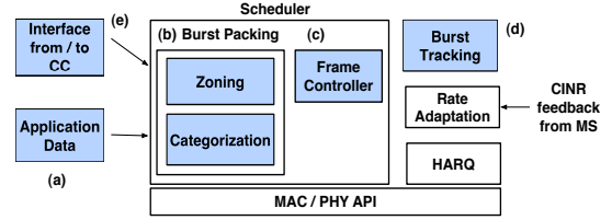
Figure 10: Implementation details of FERMI.
