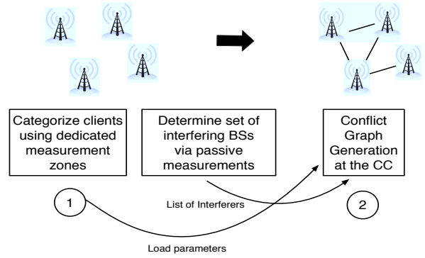
Figure 5: The building blocks of FERMI.
